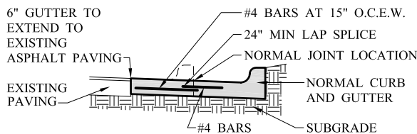
SECTION A - A CONCRETE VALLEY GUTTER FILLET NOT TO SCALE
