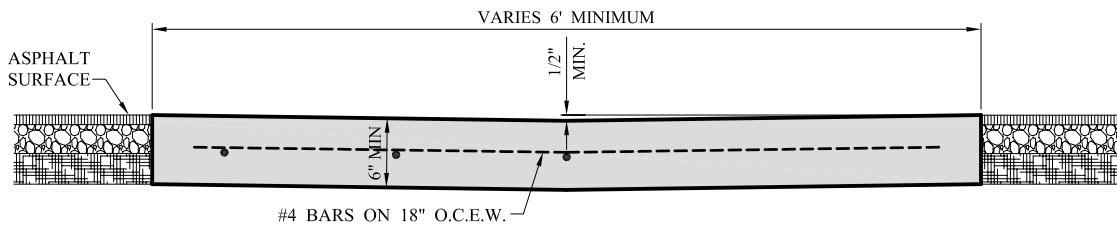
TYPICAL SECTION NOT TO SCALE
